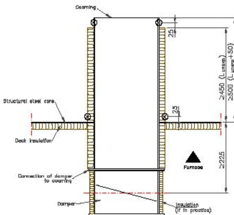
Deck specimen
