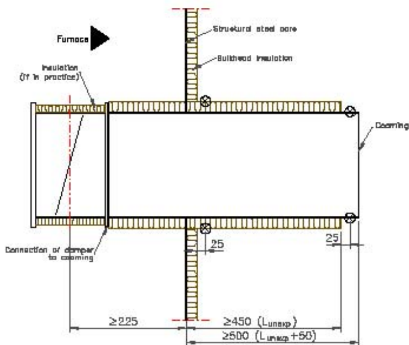
Bulkhead specimen
