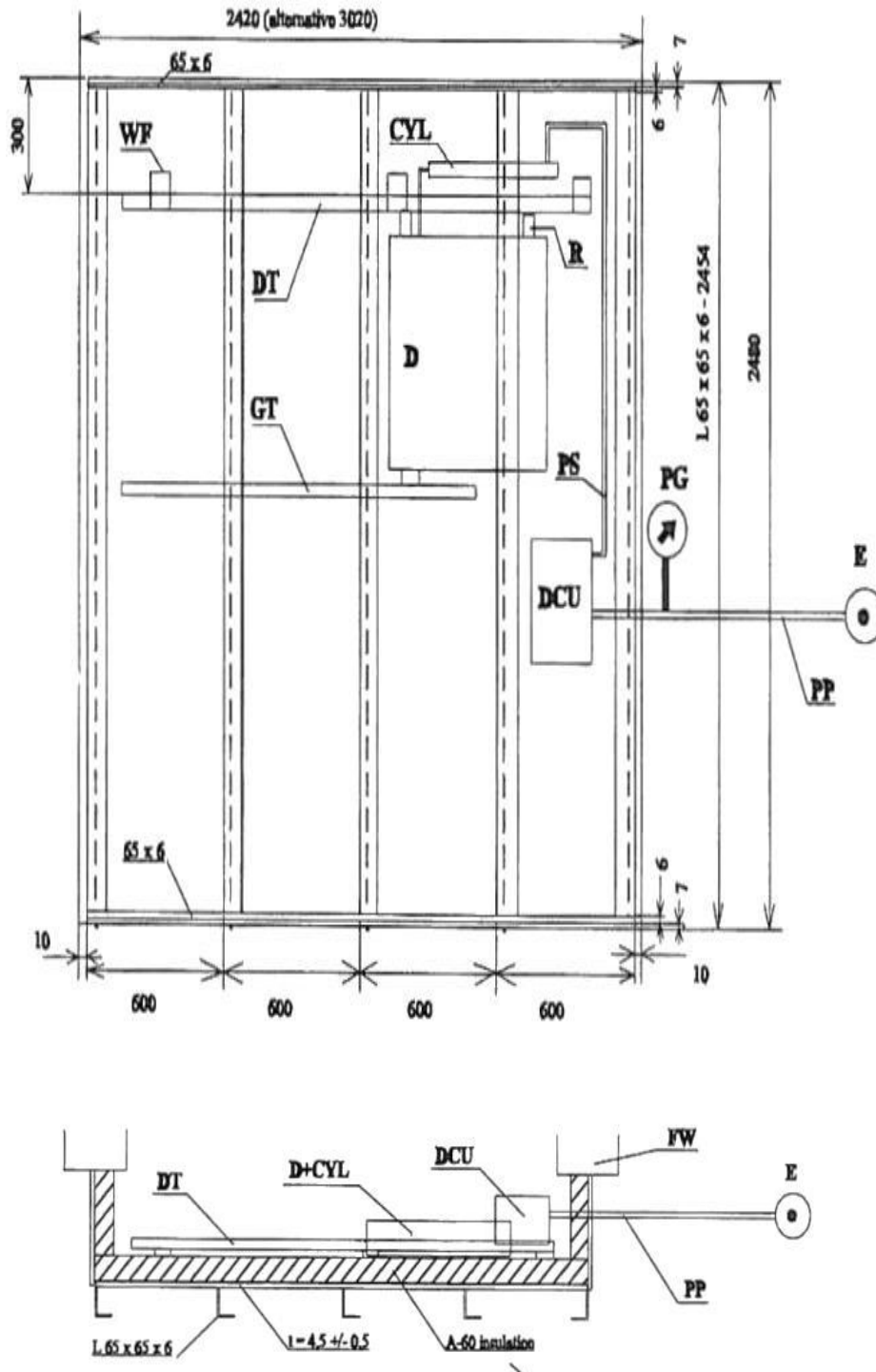
Figure 1 - Structural core for fitting the prototype fire door control system.
